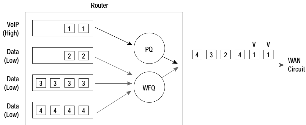
Figure 16 Optimized Queuing for Voice over IP (VoIP) over the WAN
