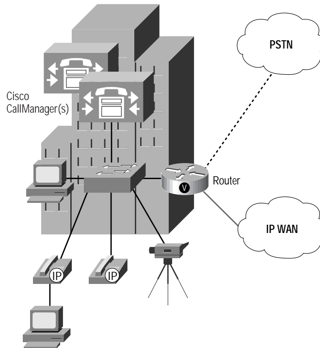
Figure 12 Enterprise Branch Office Network with Cisco AVVID
