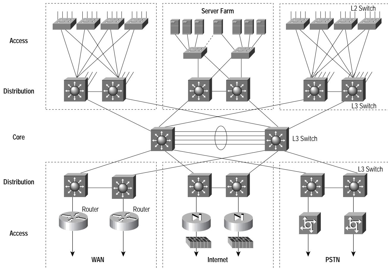
Figure 13 Enterprise Campus Network Design Model
