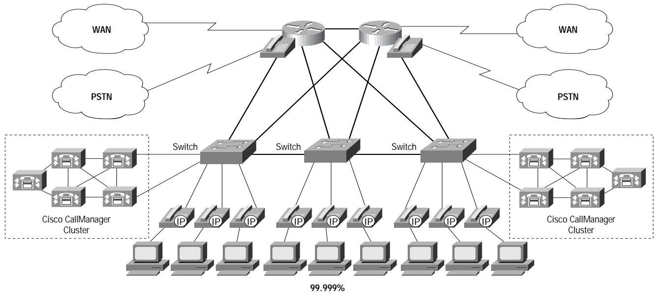
Figure 10 Network Availability
