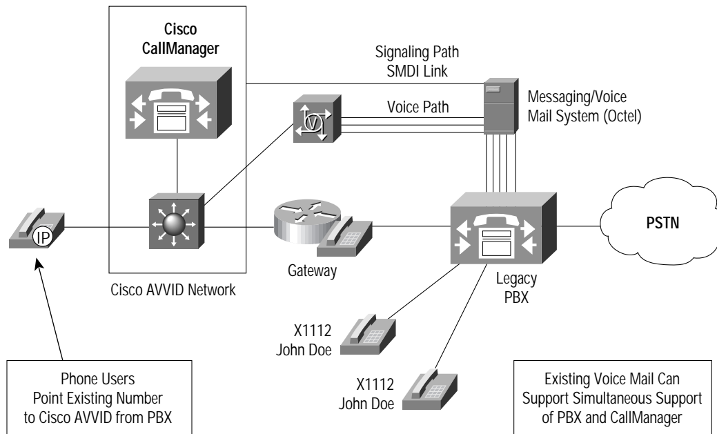
Figure 19 Migration Steps—Coexistence
